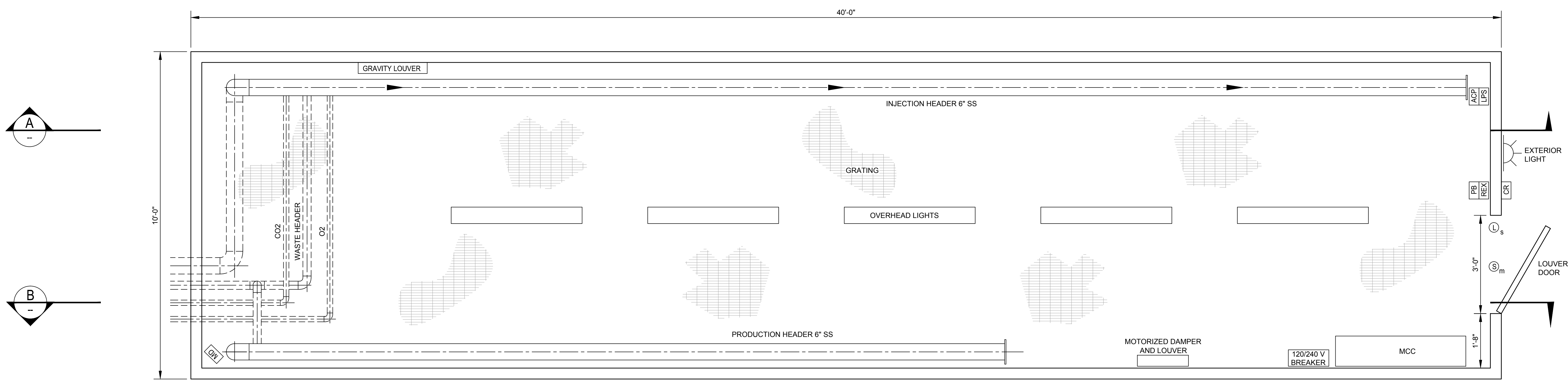
PLAN 1"=1'-6"
