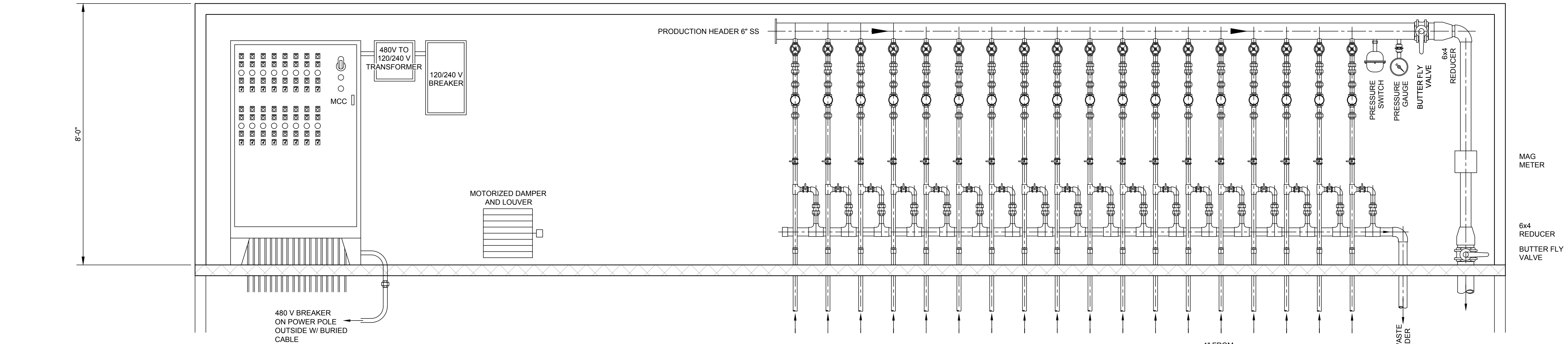
B SECTION 1"=1'-6"
